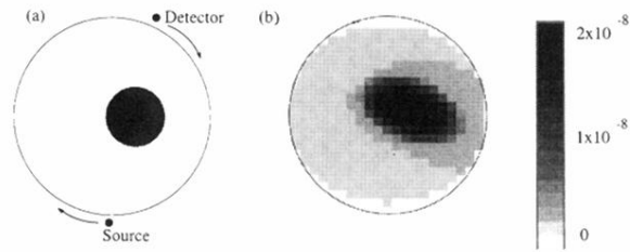
FIG. 3. An image reconstructed from experimental measurements of the scattered correlation function is shown in (b). The system was a 4.6 cm diameter cylinder with l^* = 0.25 cm, \mu_a = 0.002 cm ^{-1} , and D_B = 0 [see illustration in (a)]. A 1.3 cm diameter spherical cavity was centered at x = 0.7 cm, y = 0 , and z = 0 and filled with a colloid with l^* = 0.25 cm, \mu_a = 0.002 cm ^{-1} , and D_B = 1.5 \times 10^{-8} cm ^2 /s. A slice of the image at z = 0 cm is presented in (b). The values of the reconstructed particle diffusion coefficients are indicated by the legend in units of cm ^2 /s.
