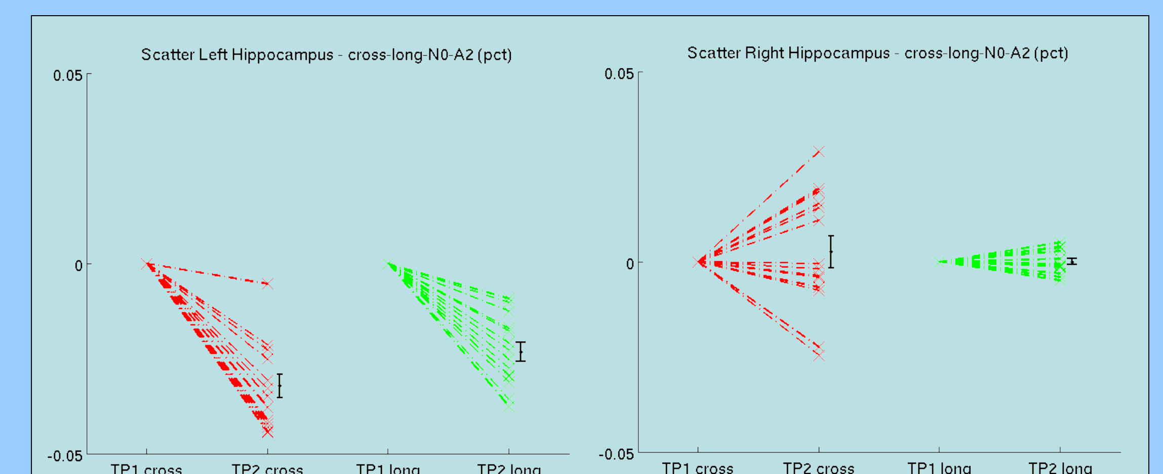
Figure 5: Left hippocampus with 2% simulated atrophy . By reducing the intensity of border voxels in the left Hippocampus, atrophy was simulated. The longitudinal processing (green) produces better results with smaller variance. Right hippocampus without any change to the image. The independently processed results (cross, red) show more variability, while the longitudinal results are highly accurate and correctly detect no change.
