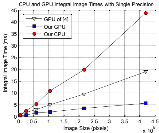
Figure 4: Performance comparison of single precision integral image computation on the CPU and the GPU. Results for [4] are replicated from their work
